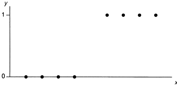
Figure 5.3. Perfect discrimination resulting in infinite logistic regression parameter estimate.
